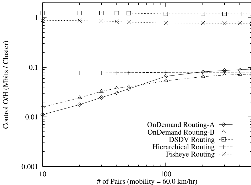
Figure 4: Control O/H vs. Traffic Pairs
