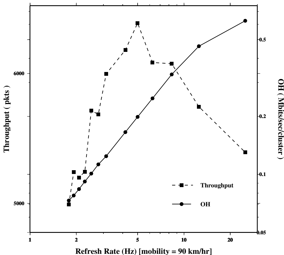
Figure 8: Soft state evaluation (90 km/hr)
