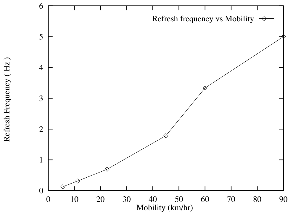
Figure 9: Refresh Rate vs. Mobility
