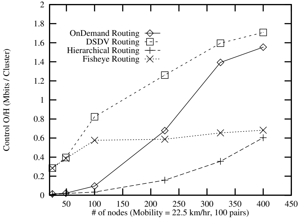
Figure 10: Control O/H vs. number of nodes
