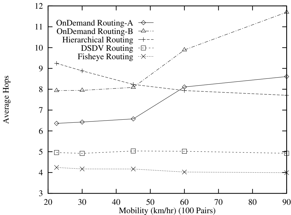
Figure 7: Average Hops vs. Mobility (100 Pairs)
